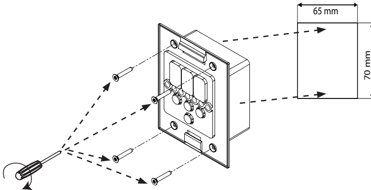
Fig. 5 Installing the Pro D control panel
