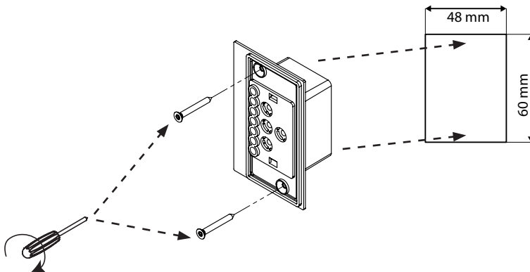
Fig. 6 Installing the control panel additional output (optional)
